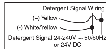
Figure 7 Detergent Signal Wiring – Probe or Probeless
