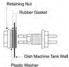
Figure 3 Probe Mounting
