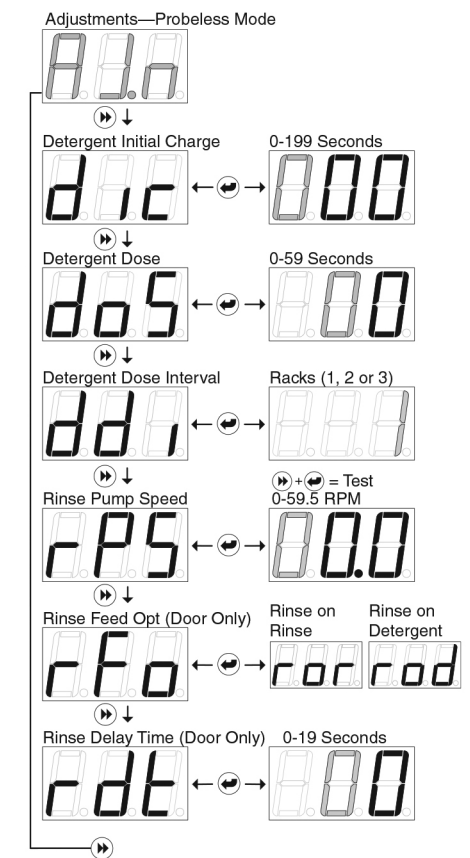
Figure 15 Adjustments - Probeless Mode (Menu Adj.n )
