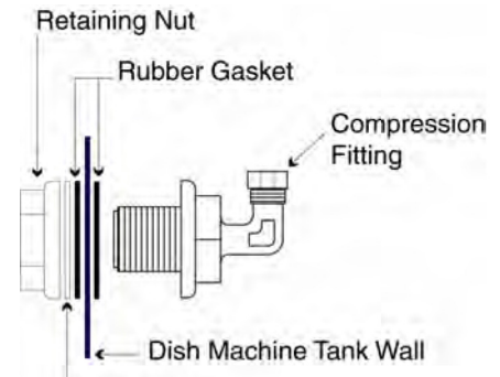
Figure 5 Detergent Bulkhead Fitting
