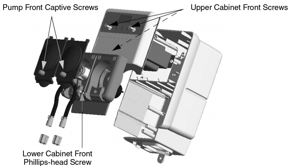
Figure 17 Sprite Cabinet Assembly
