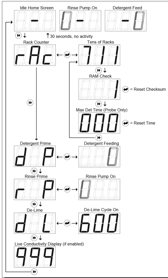
Figure 10 User Mode Menus and Displays
