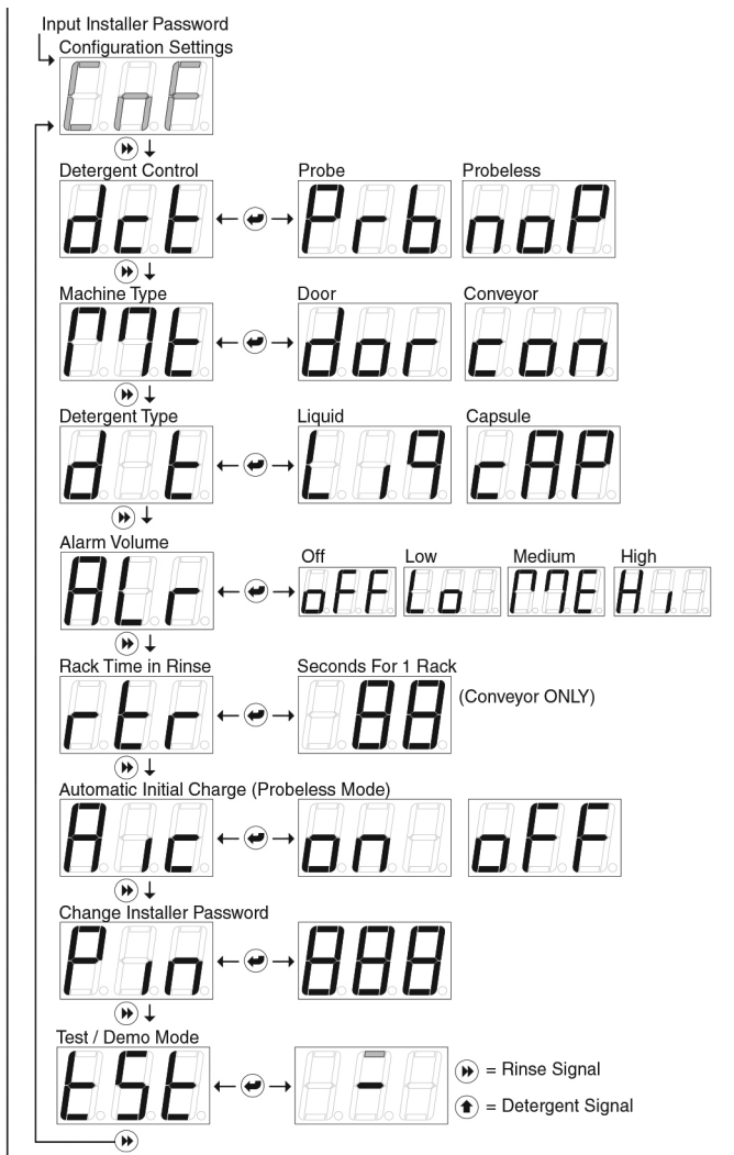
Figure 13 Configuration Settings (Menu \underline{CnF} )
