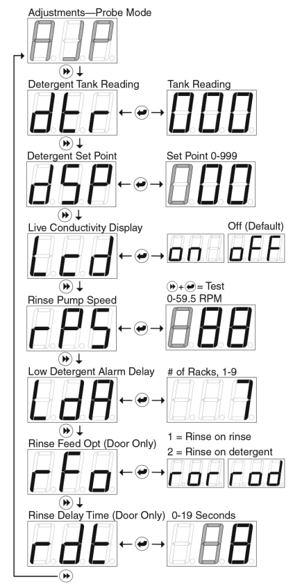
Figure 14 Adjustments - Probe Mode (Menu AJ.P )
