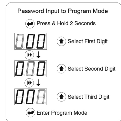
Figure 11 Program Mode Access
