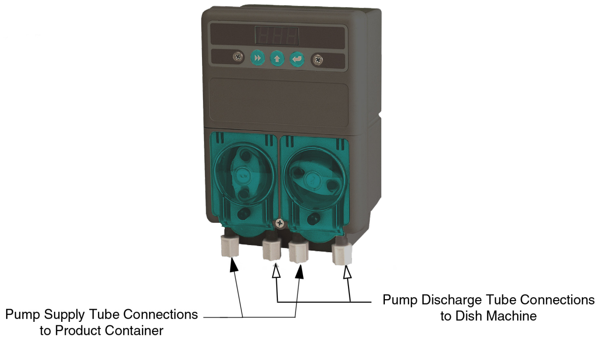
Figure 6 Sprite DM 420 Tube Connections
