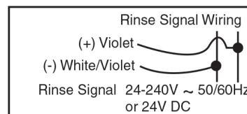
Figure 8 Rinse Signal Wiring – Probe or Probeless
